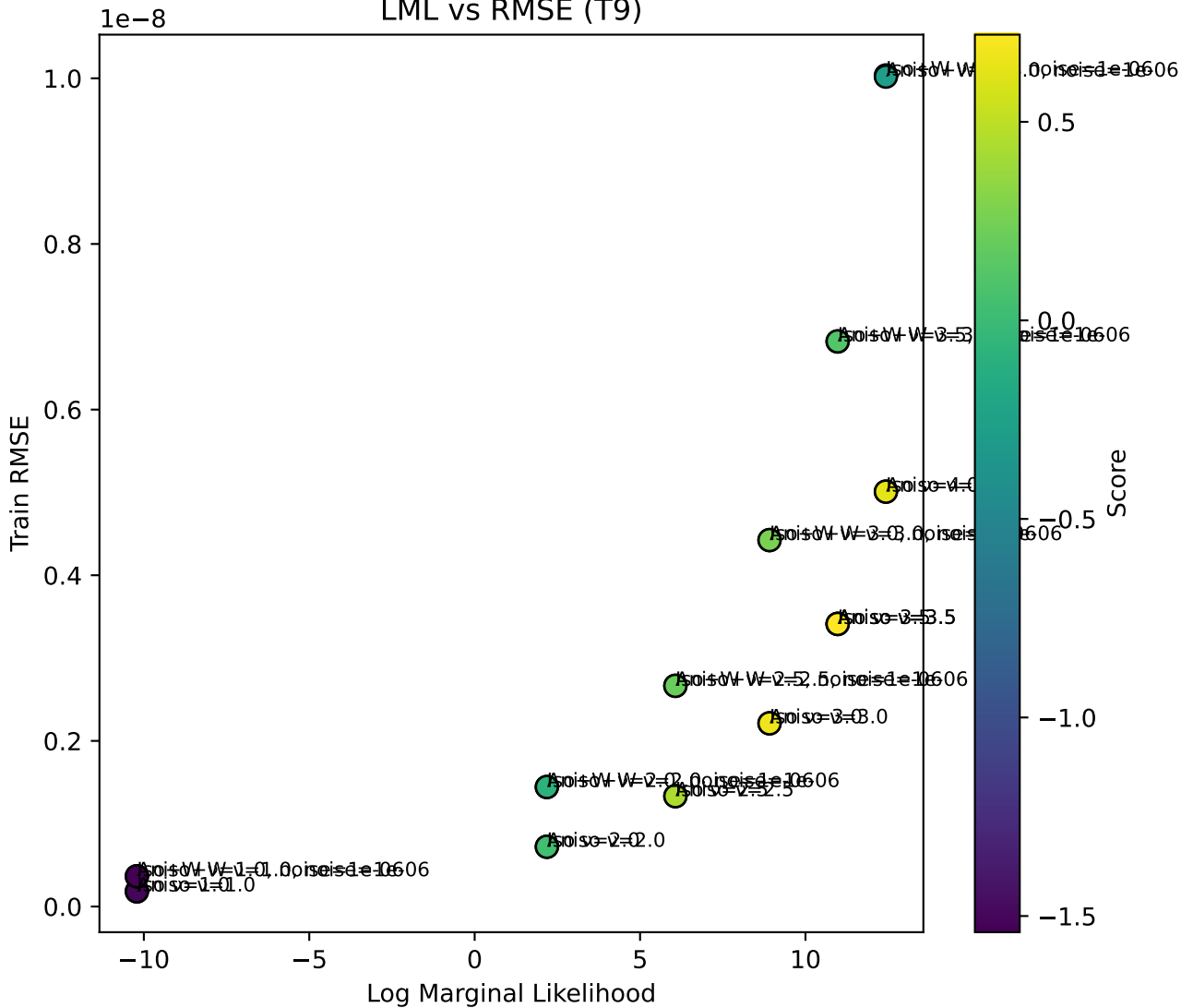
LML vs RMSE (T9)
