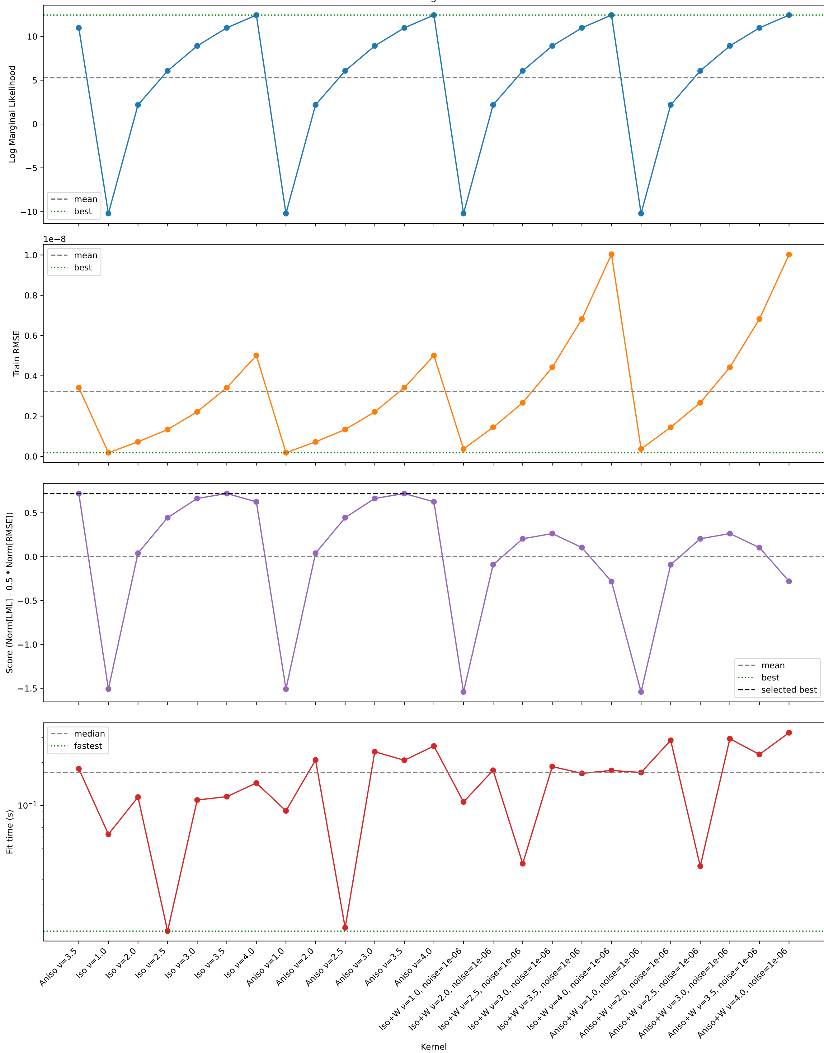
Kernel diagnostics T9
