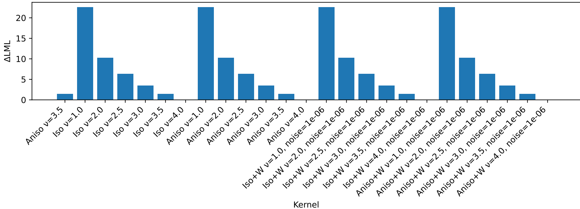
Difference from best LML (T9)
